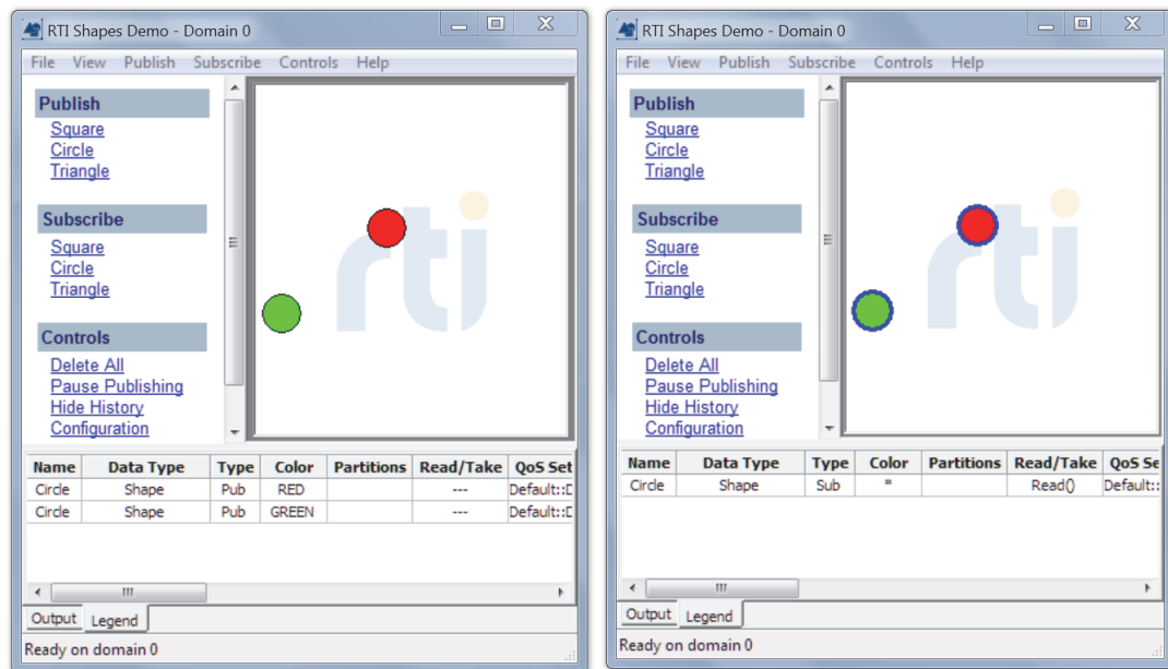
Publisher1
