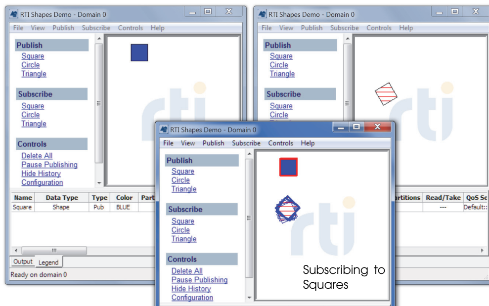
Publishing “Shape”
