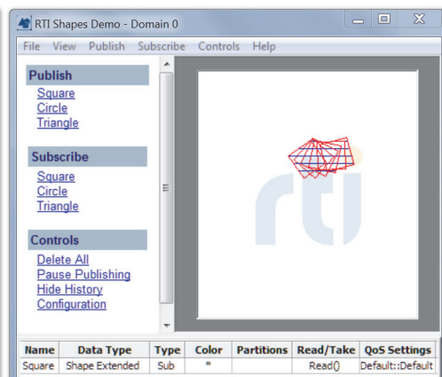
Subscriber1
