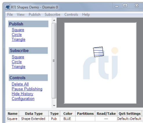
Publisher1
