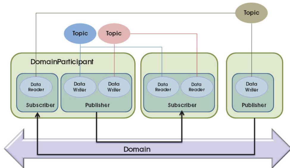
Figure 3.1 DDS Components
