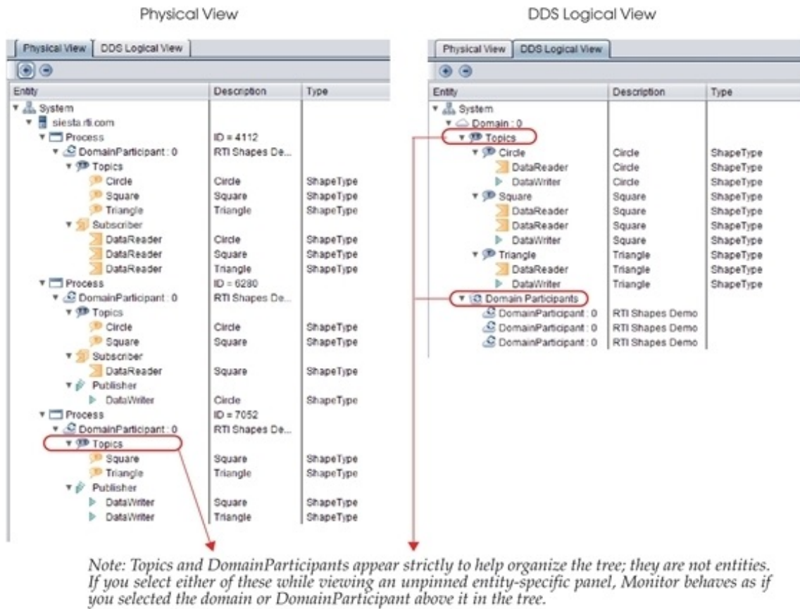
Figure 3.1: Physical and DDS Logical Views
