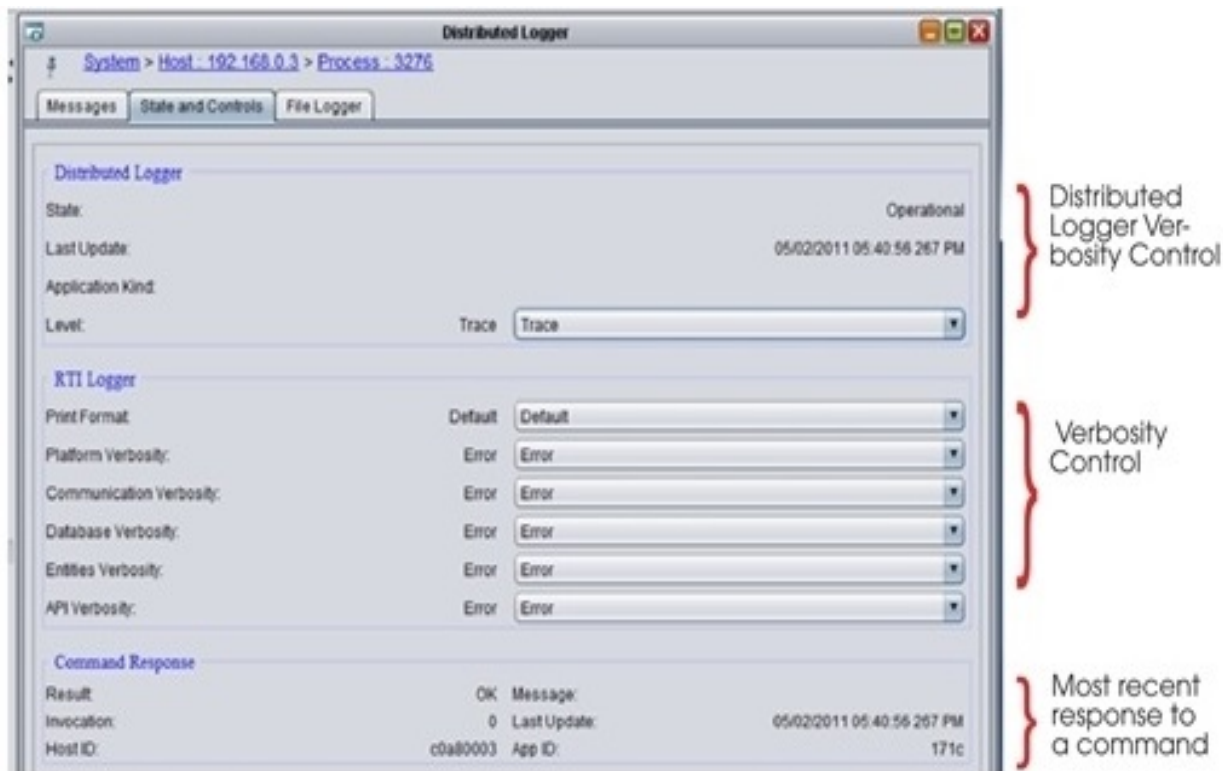
Figure 3.11: Distributed Logger Panel's State and Controls Tab
