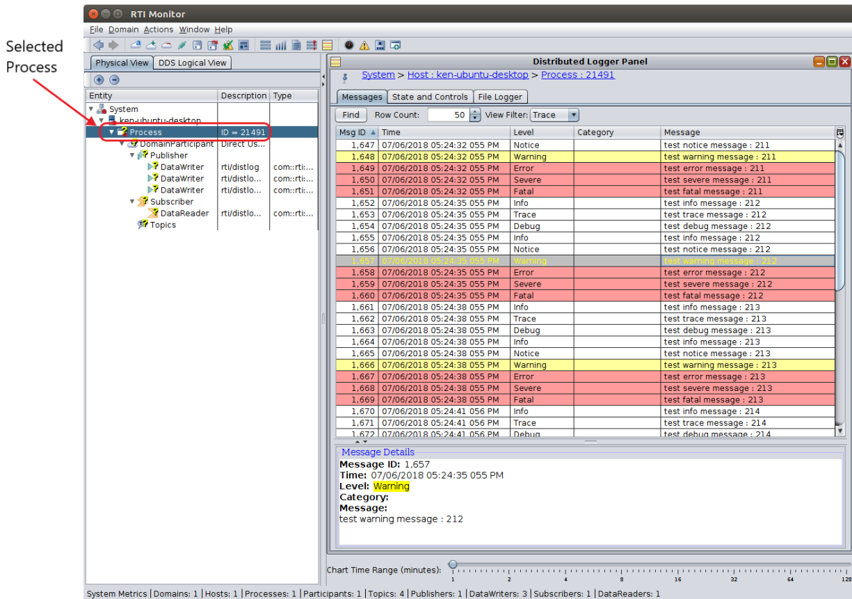
Figure 3.9: Distributed Logger Panel
