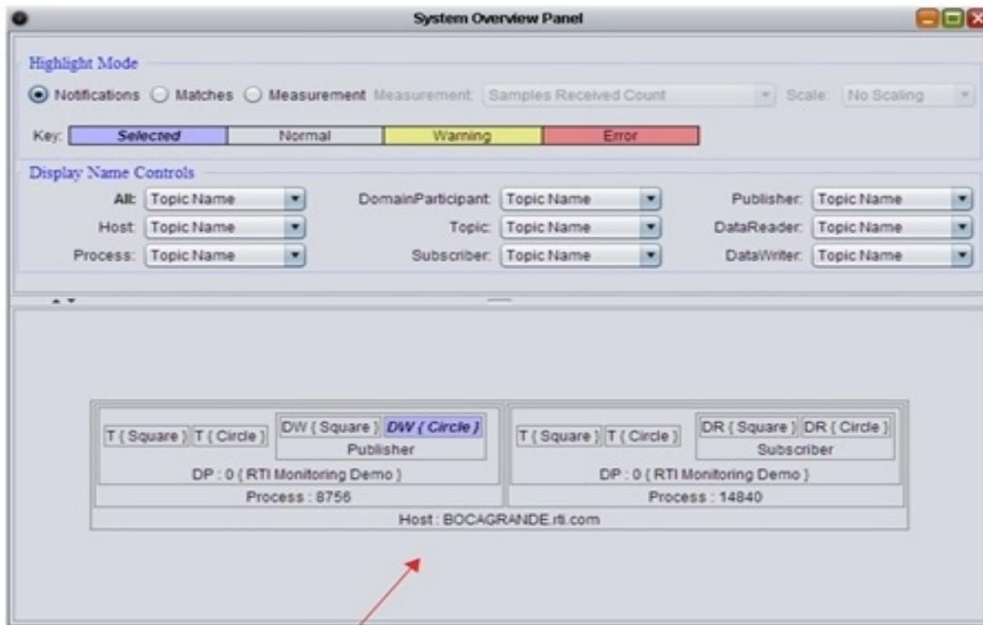
Figure 3.13: System Overview Panel (Notifications Option)
