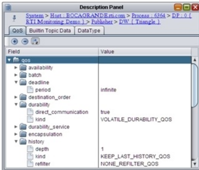
Figure 3.4: Description Panel's QoS Tab
