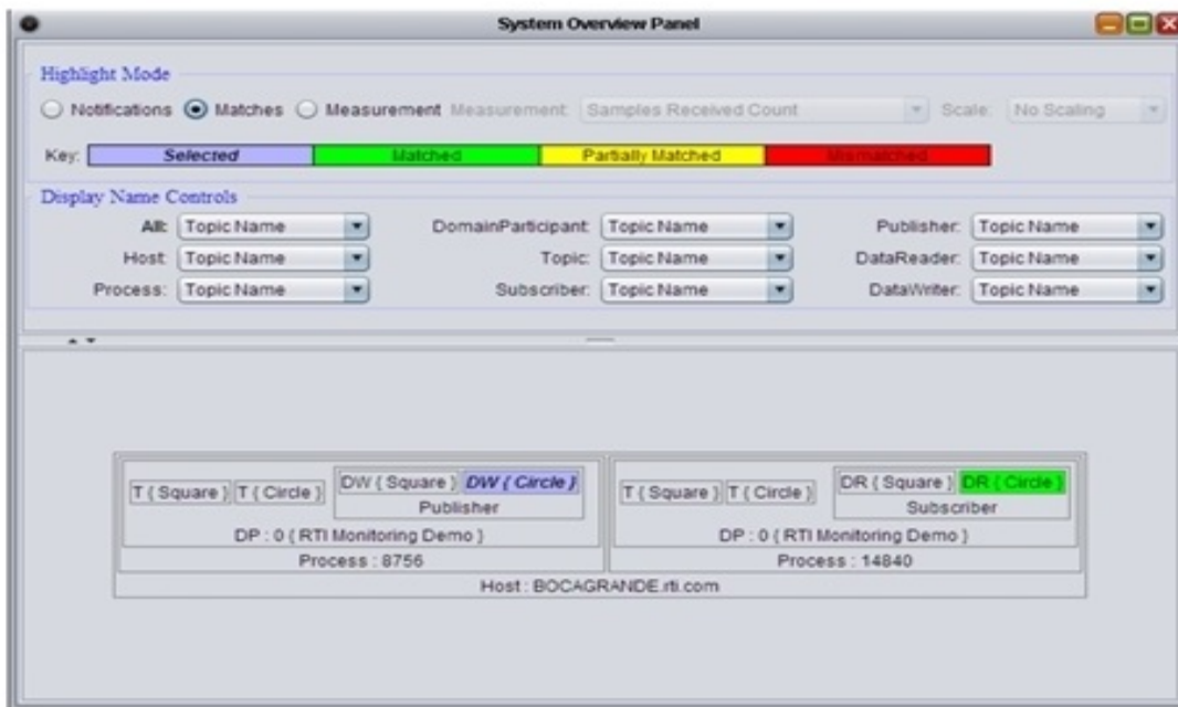
Figure 3.14: System Overview Panel (Matches Option)
