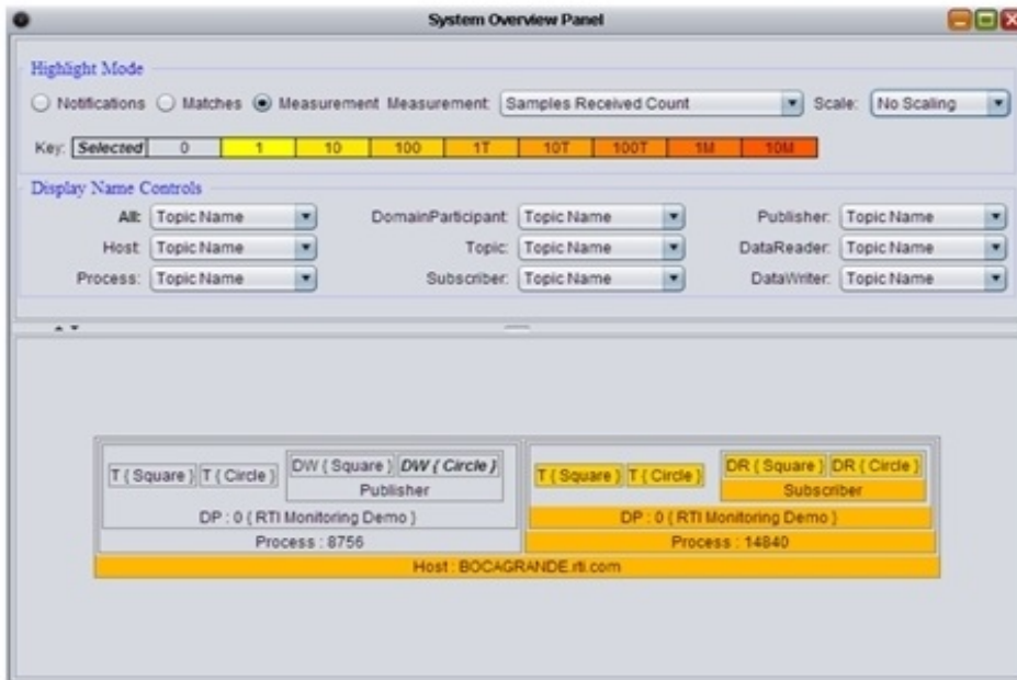
Figure 3.15: System Overview Panel (Measurement Option)
