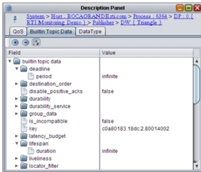
Figure 3.5: Description Panel's Builtin Topic Data Tab
