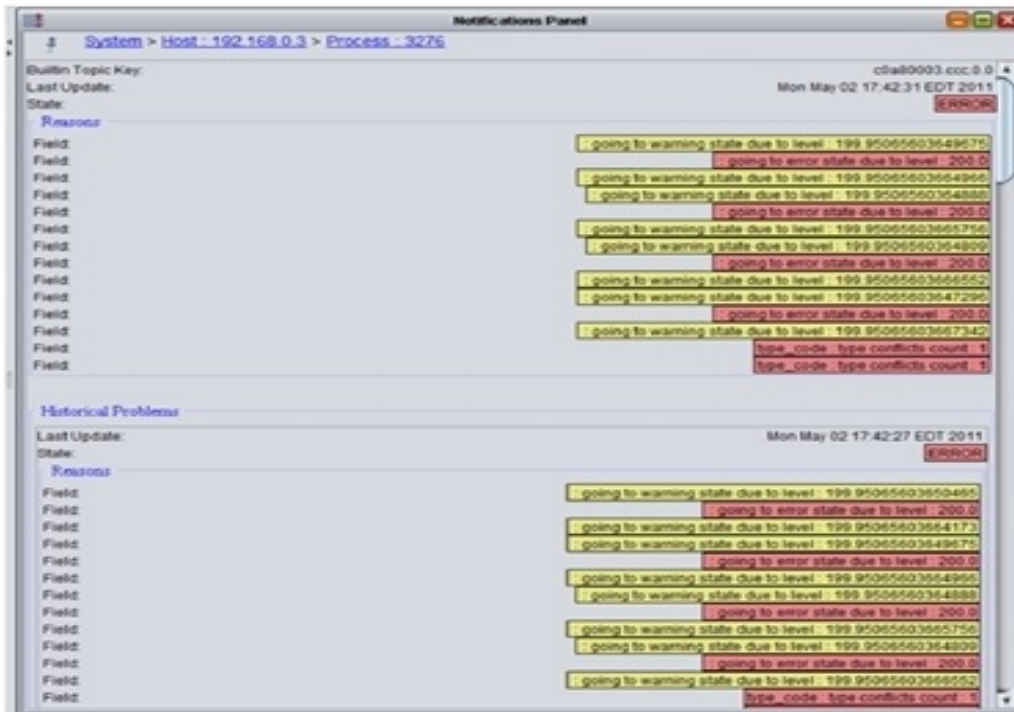
Figure 3.8: Notifications Panel: Integrating Log Message Level with Entity State
