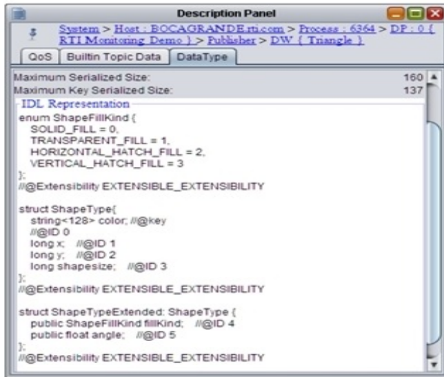
Figure 3.6: Description Panel's Data Type Tab
