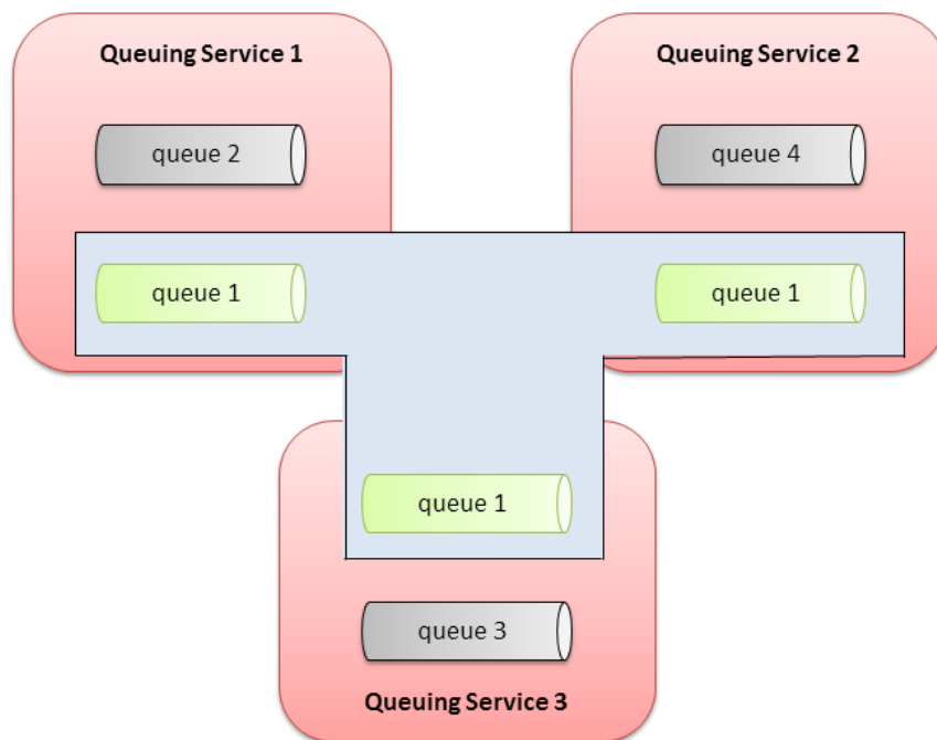
Figure 7.1: Replicating SharedReaderQueues
