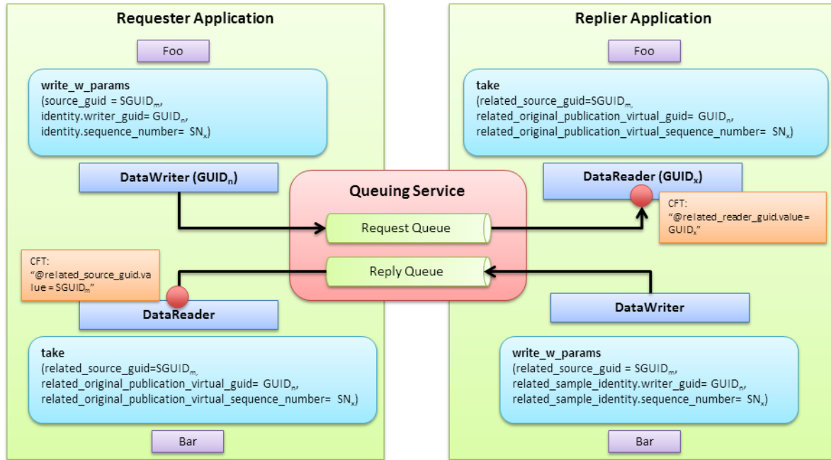
Figure 2.6: Request Generation
