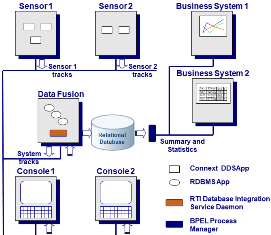
Figure 2.1: Example System Using Database Integration Service
