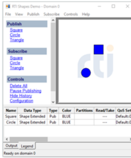
Publisher1 NonSecure
