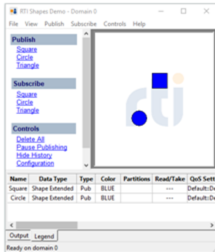
Publisher1 NonSecure
