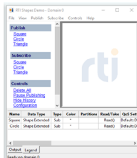
Participant1 SecureAllowAll
