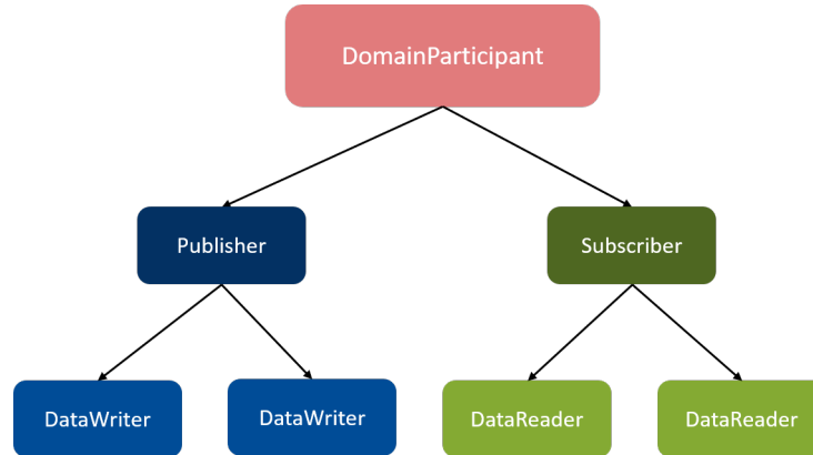
Figure 3.5: DomainParticipants create and manage Publishers and Subscribers . Publishers create and manage DataWriters . Subscribers create and manage DataReaders . DataWriters and DataReaders send and receive your data.
