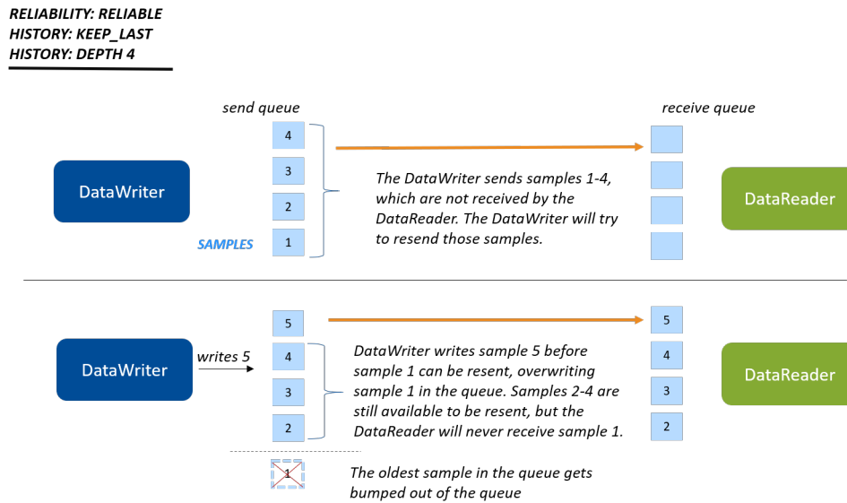
Figure 5.5: Keep-Last Reliability (unkeyed or with a single instance): In this example, you have four slots open on the writer side to keep samples that have not yet been received by the reader.
