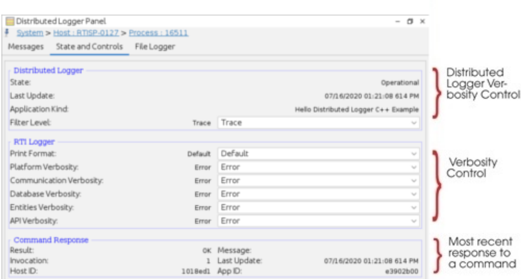
Figure 3.11: Distributed Logger Panel's State and Controls Tab
