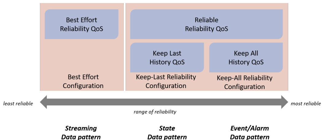
Figure 5.7: A range of reliability options between Best Effort and Reliable. If a RELIABLE kind is selected, the History QoS Policy comes into play.
