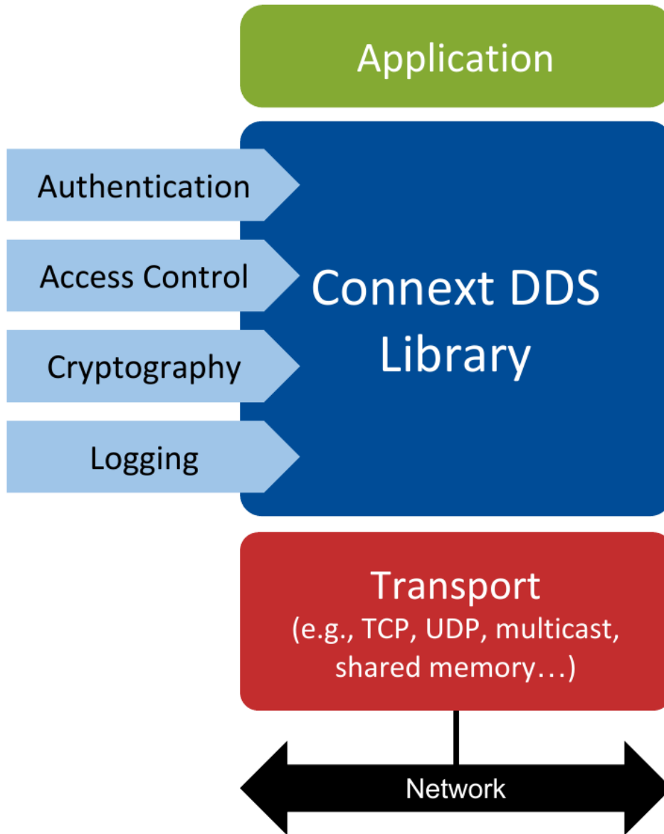
Figure 1.1: Architecture of an application using SECURITY PLUGINS. All the currently available security plugins (Authentication, Access Control, Cryptography and Logging) are implemented in a single nddssecurity library.
