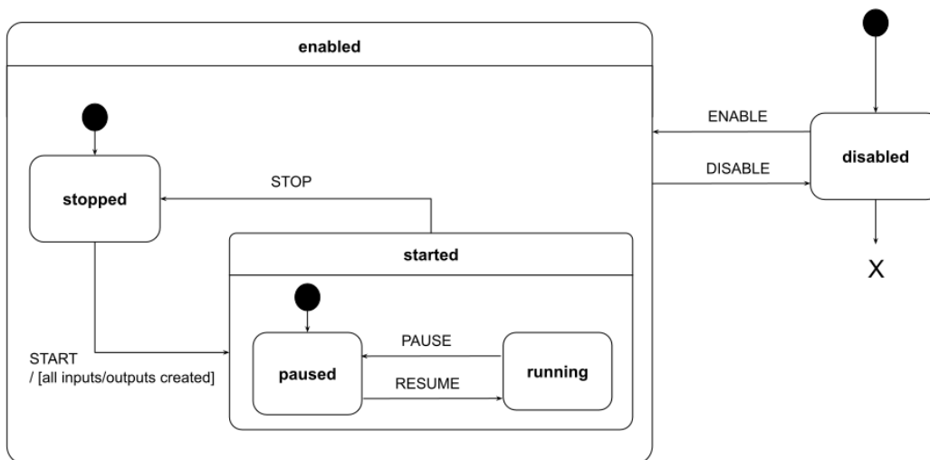
Figure 11.8: Route state machine
