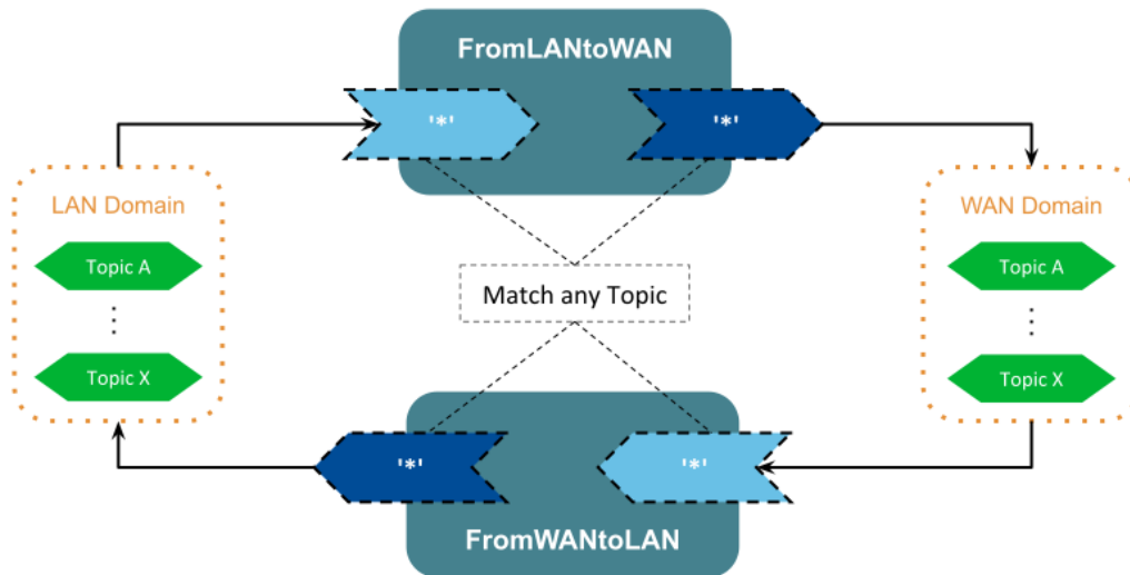
Figure 3.12: Definition of AutoTopicRoute to forward topics bidirectionally
