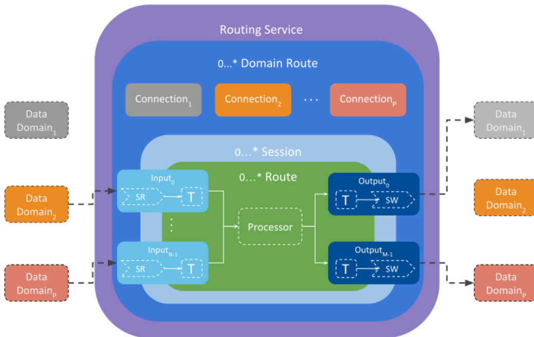
Figure 11.2: Routing Service Alternative representation of the Application Resource Model
