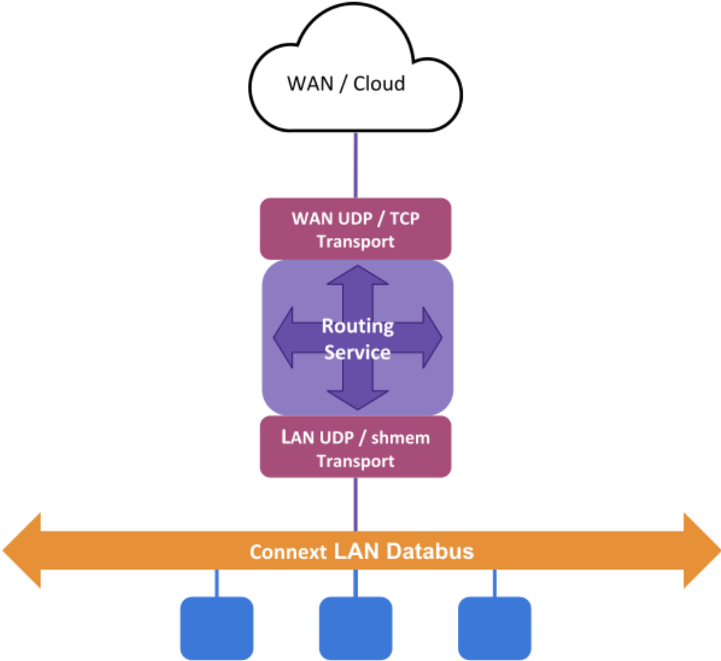
Figure 3.9: Routing Service as WAN/Cloud gateway
