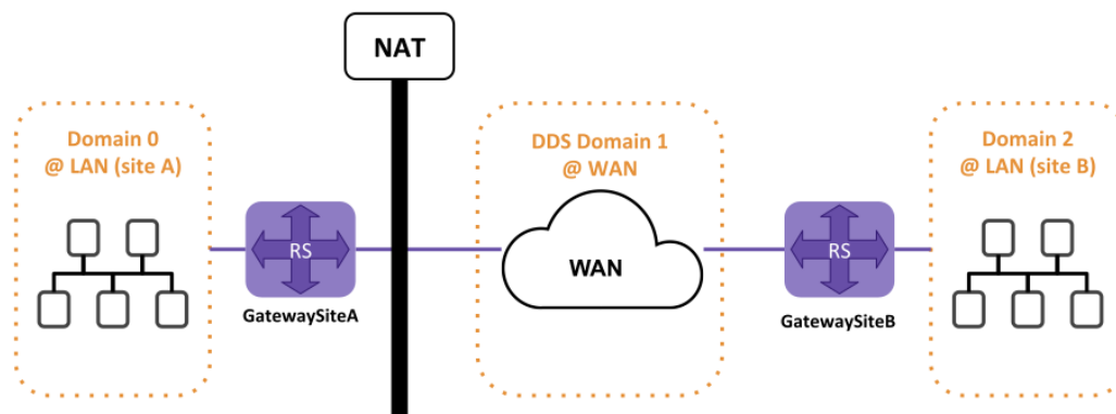
Figure 14.1: Example using the TCP transport to traverse WAN
