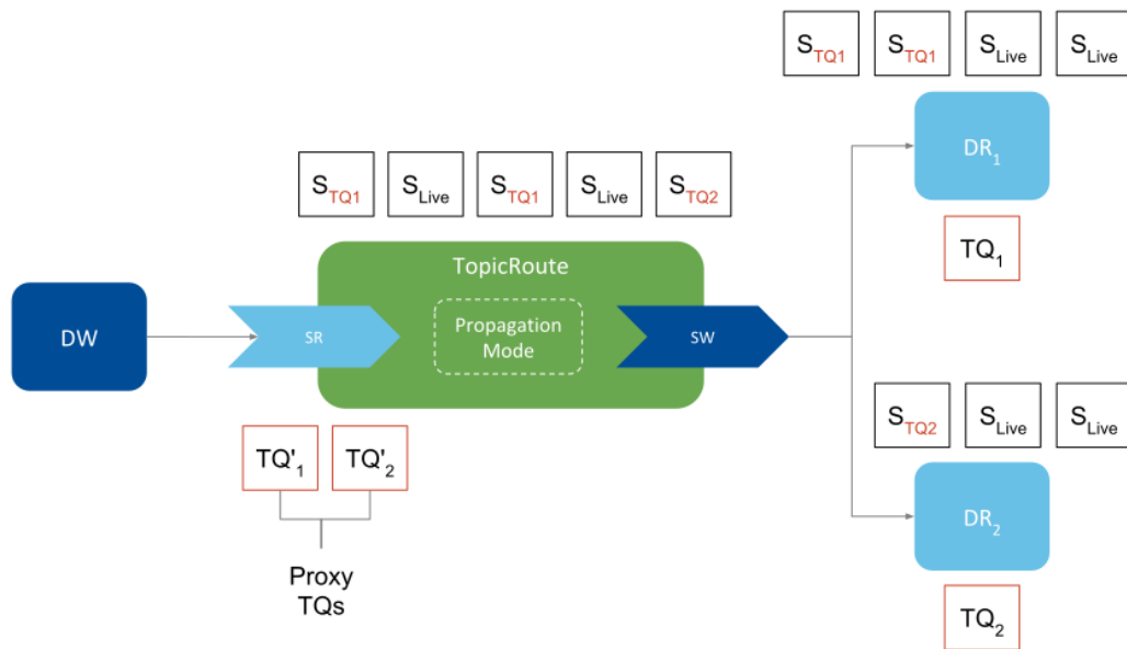
Figure 12.6: TopicRoute Enabling TopicQuery Proxy in Propagation Mode
