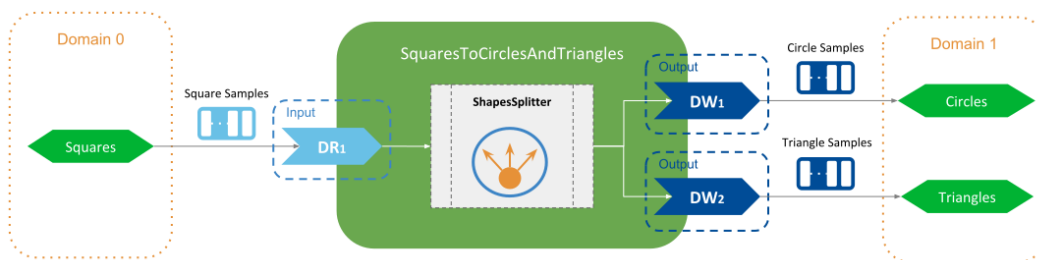
Figure 4.5: Splitting example of a Topic
