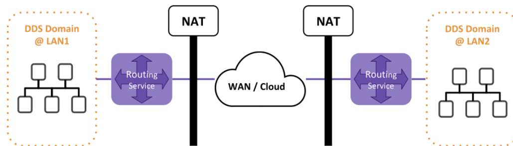
Figure 3.8: WAN traversal with Routing Service .
