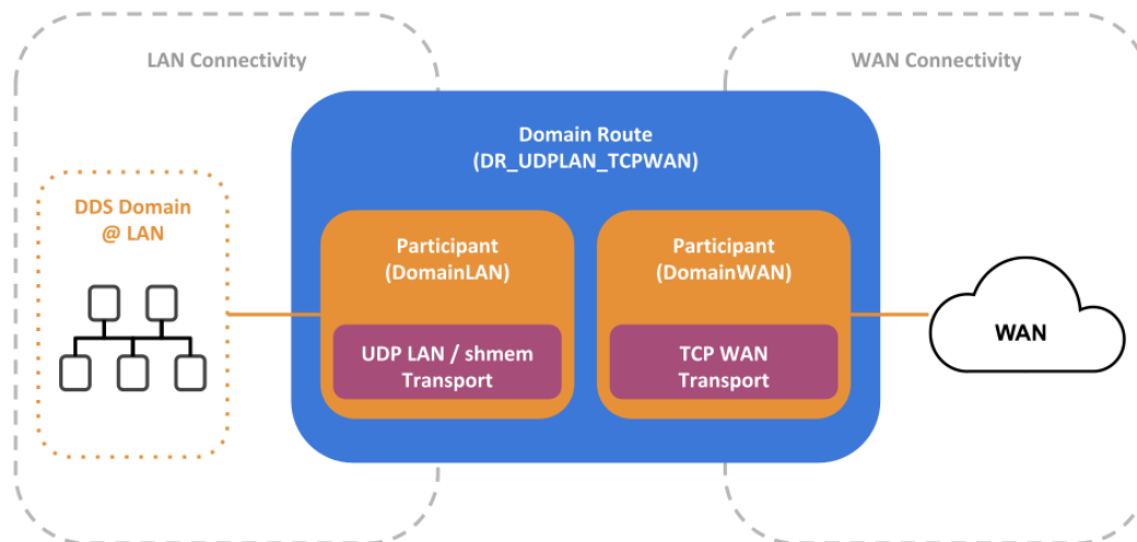
Figure 3.11: Configuration of the DomainRoute to forward data over the WAN
