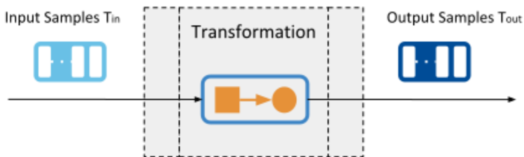
Figure 4.6: Transformation concept
