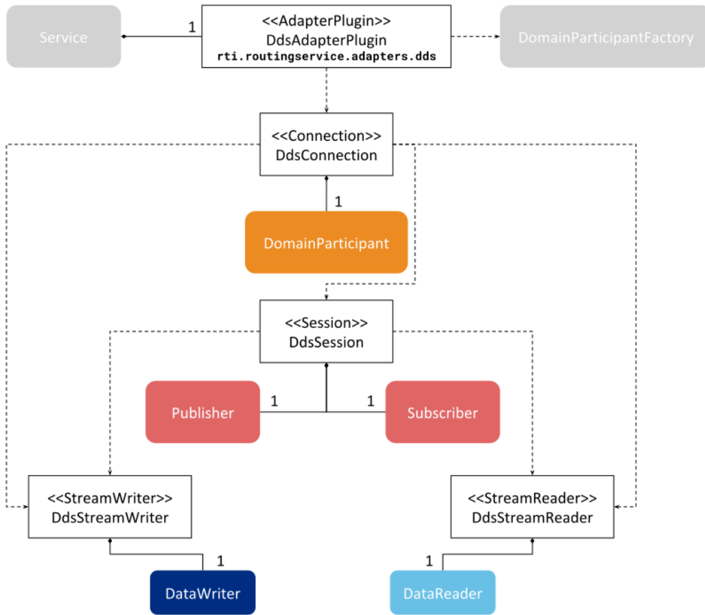
Figure 11.12: DDS Adapter architecture
