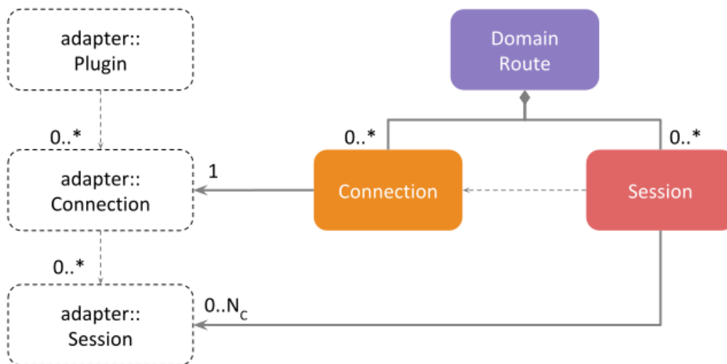
Figure 11.6: Relationship of plugins with a Session
