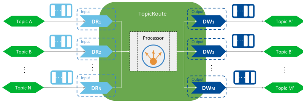
Figure 4.2: Processor concept
