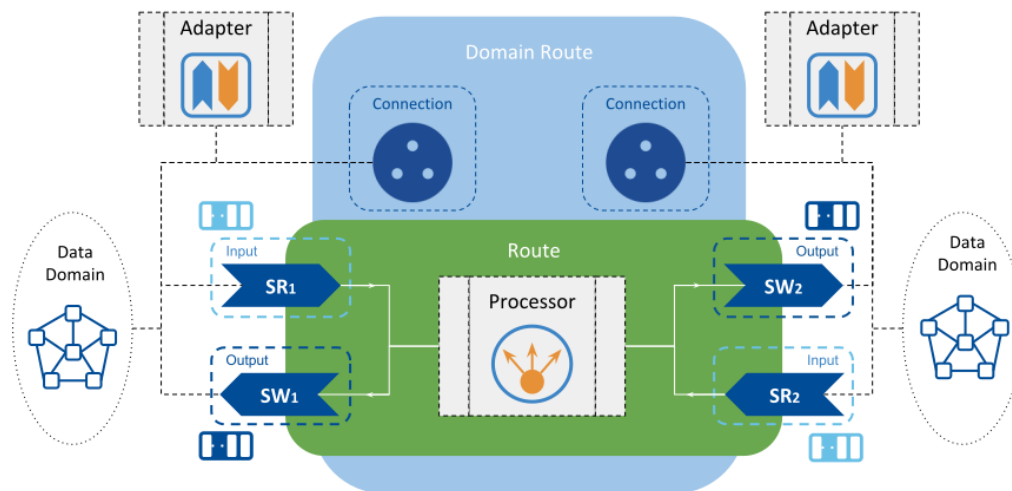
Figure 5.2: Adapter concept
