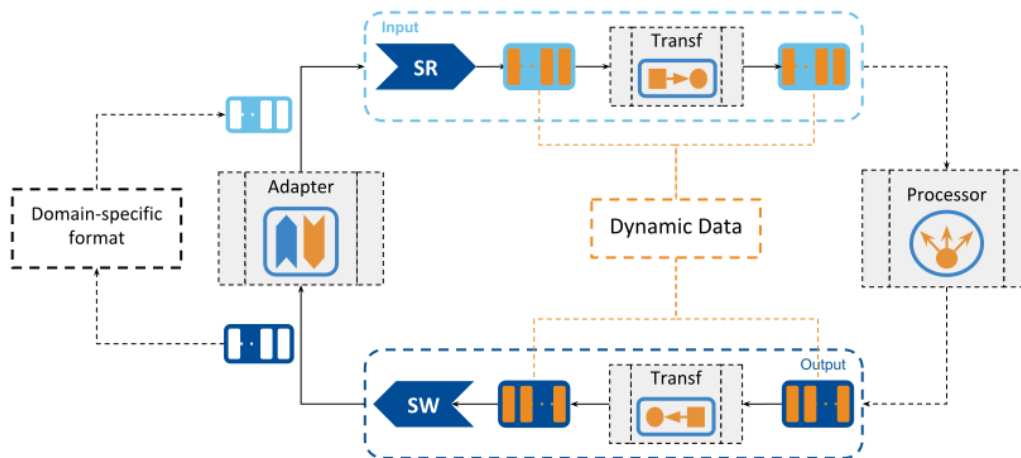
Figure 5.3: Unified Data Representation Model
