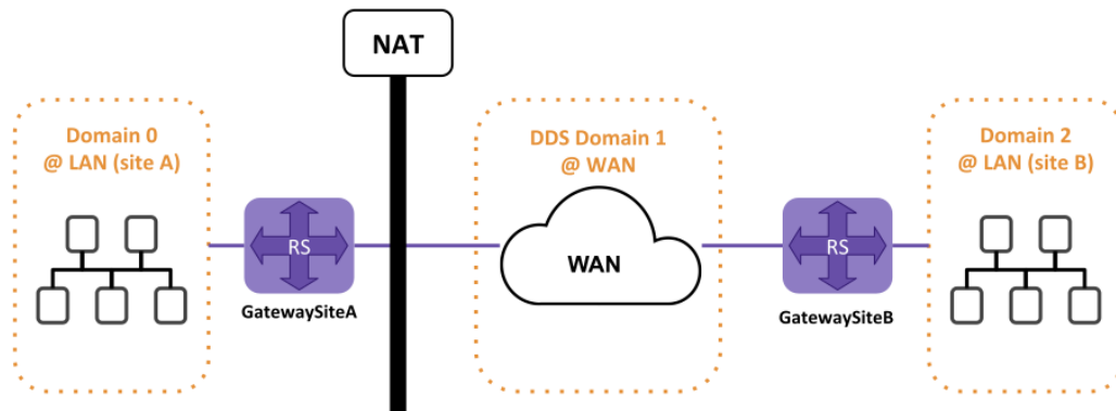
Figure 3.10: Example using the TCP transport to traverse WAN
