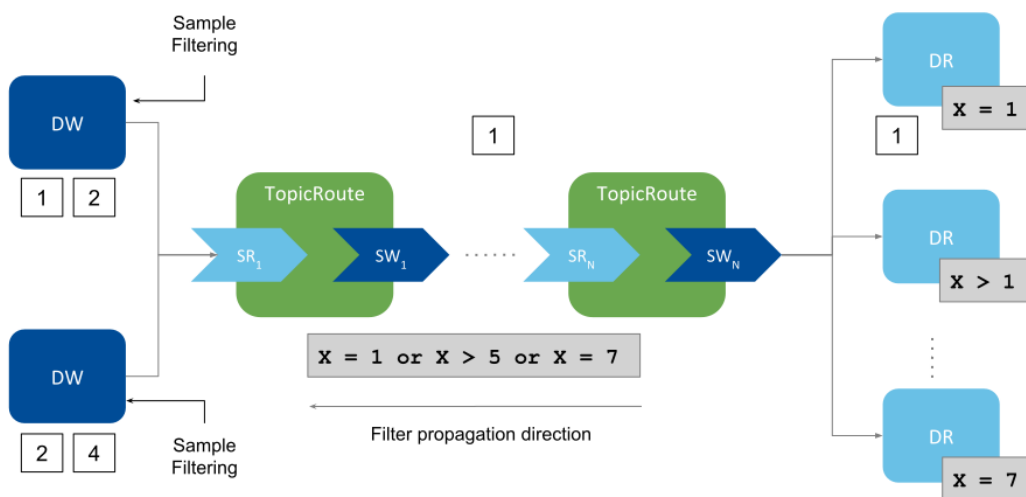
Figure 12.2: With propagation, user Data Writers receive a composed filter that allows writer-side filtering, thus sending only the samples of interest to the Data Readers
