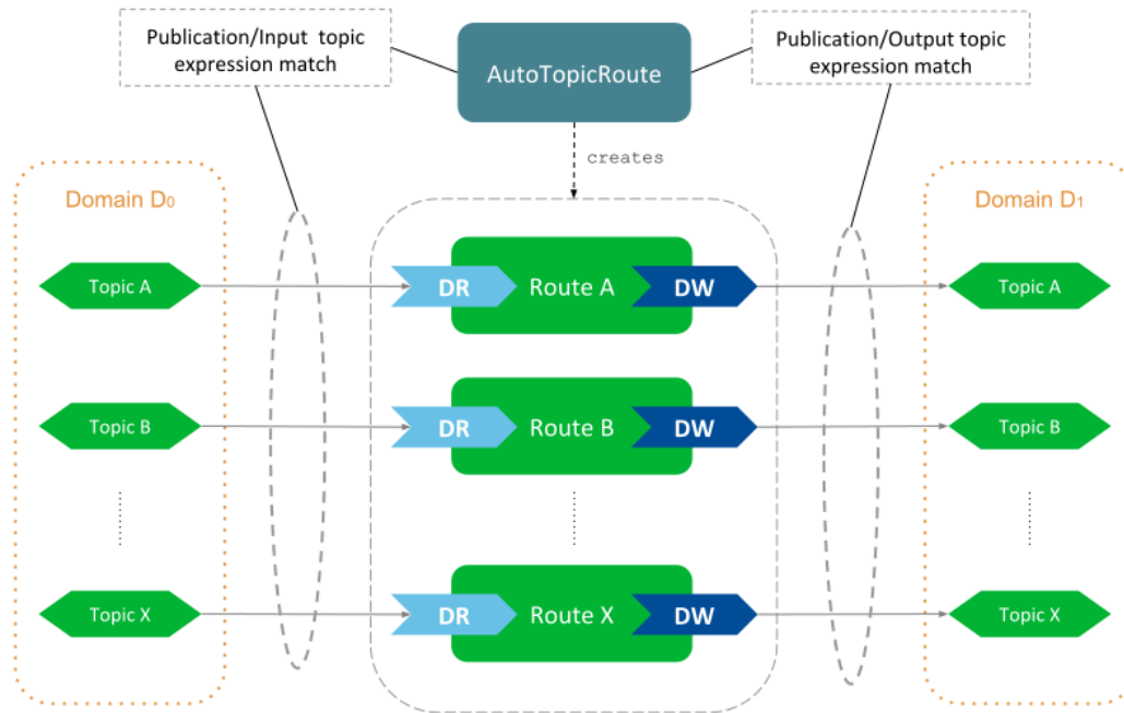
Figure 3.6: AutoTopicRoute concept
